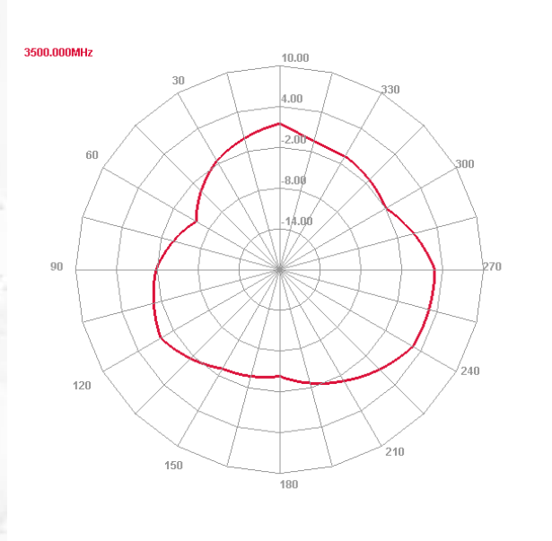
H plane
