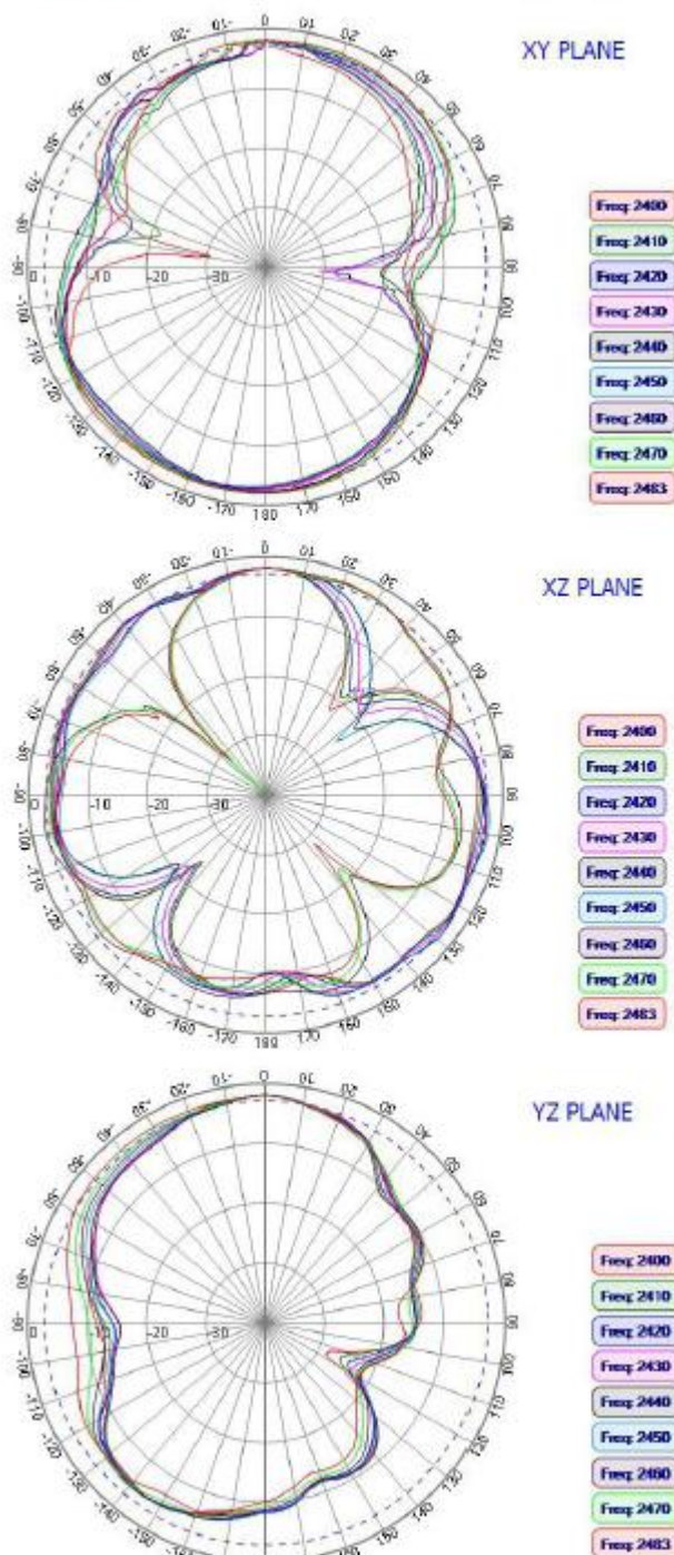
WIFI Antenna
