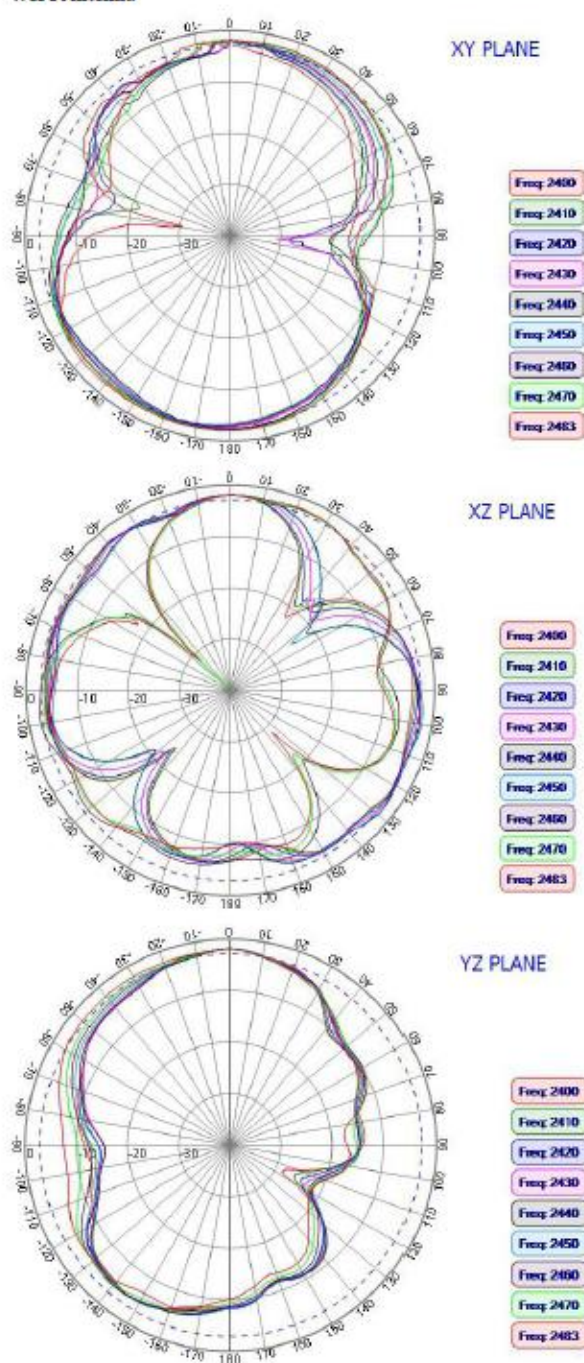
WIFI Antenna
