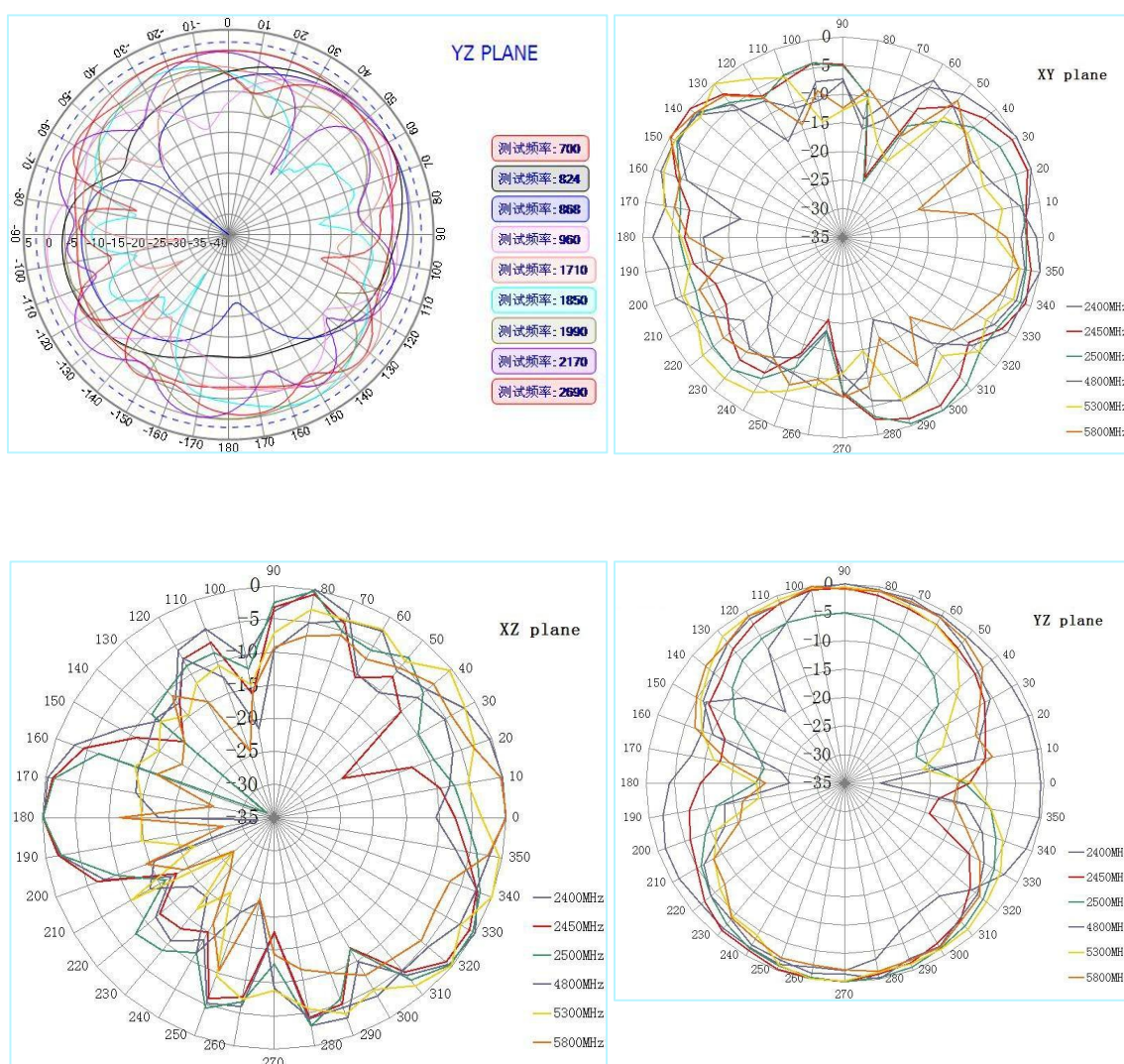
WIFI Antenna
