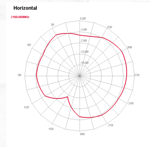
2100 MHz H plane
