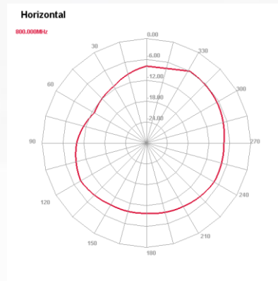
800 MHz H plane
