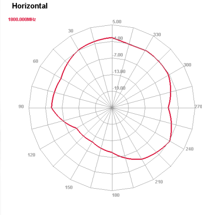
1800 MHz H plane
