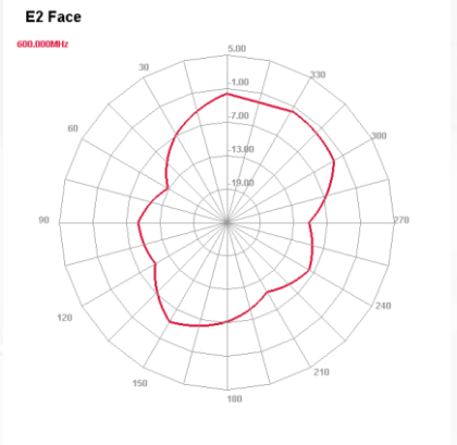
600 MHz E plane
