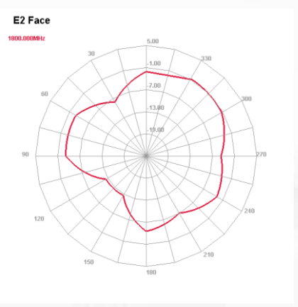
1800 MHz E plane
