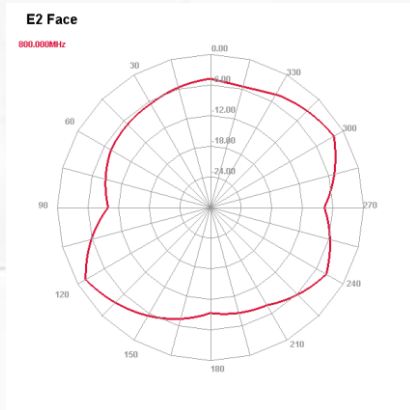
800 MHz E plane
