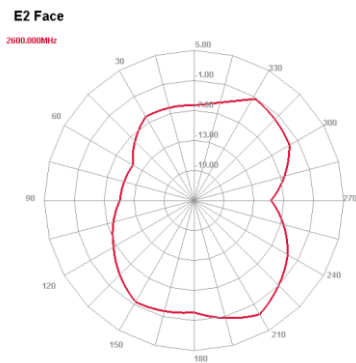
2600 MHz E plane
