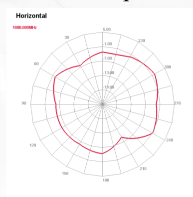
1800 MHz H plane
