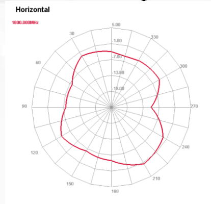
1800 MHz H plane
