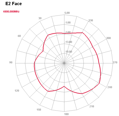
4800 MHz E plane
