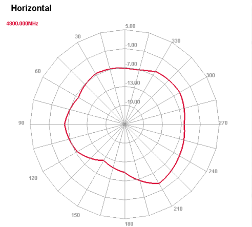
4800 MHz H plane
