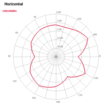
2600 MHz H plane
